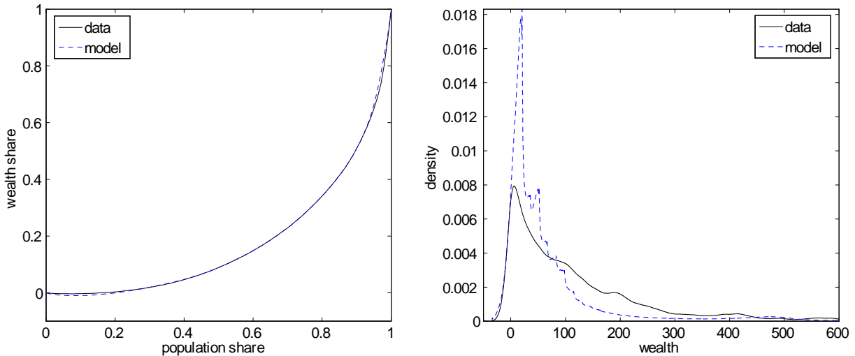
Figure 9 Fit of the (targeted) Lorenz curve and the corresponding fit of the (non-targeted) density in 2008
