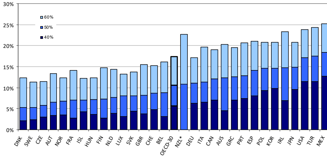
Figure 13 Poverty rates in OECD countries
