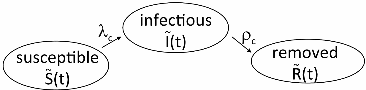
Abbildung 65 Transition between states in the classic SIR model
